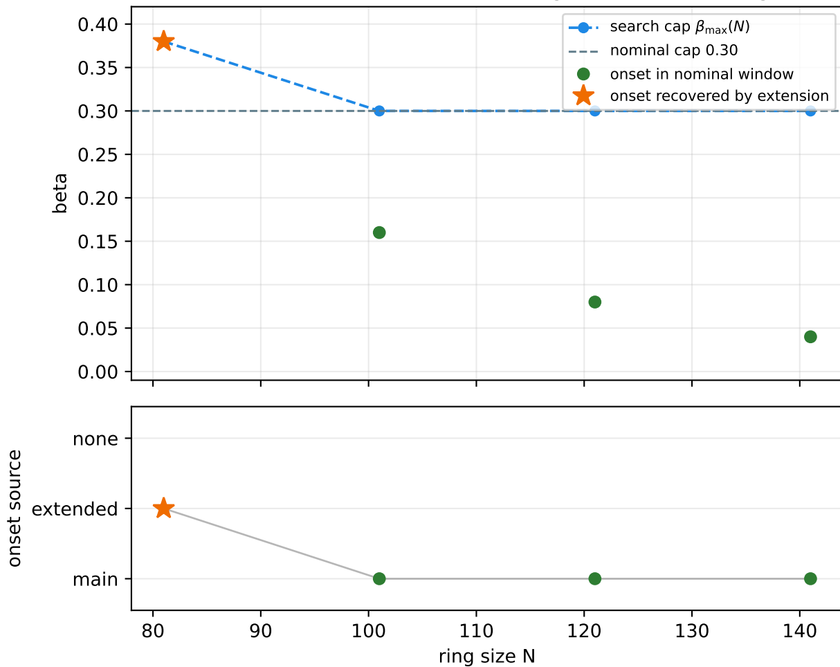
Onset source and search-window diagnostics across ring sizes
