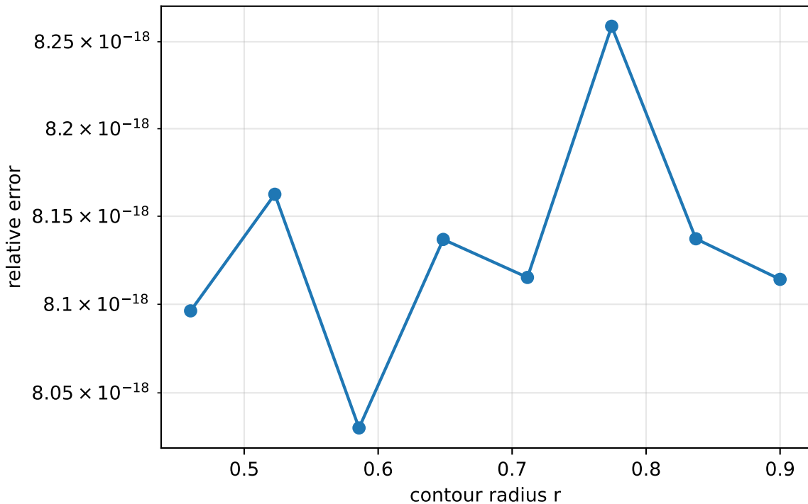
A1/A8 radius invariance in admissible annulus
