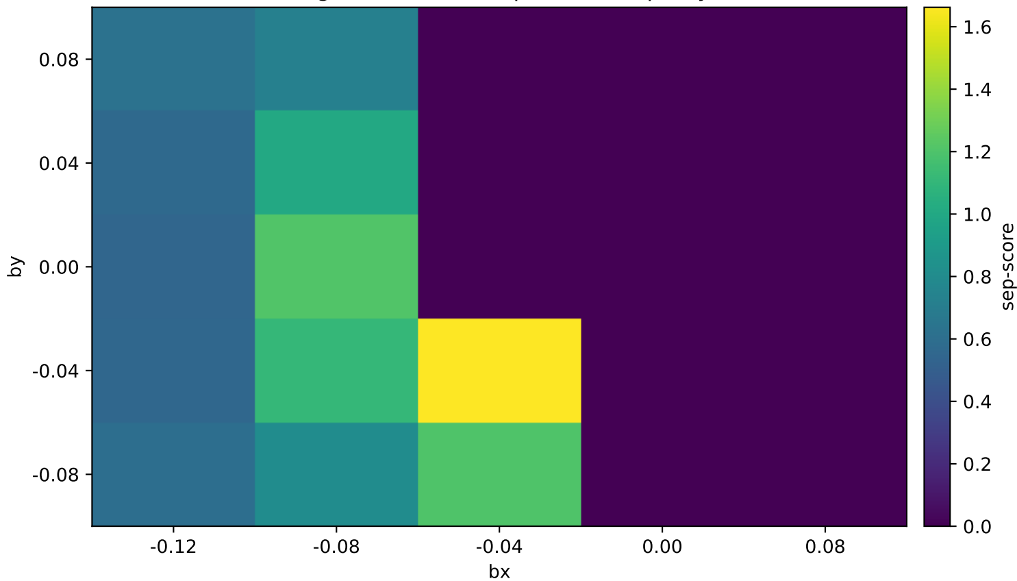
One-target bias-vector separation map ( W_y=12 )
