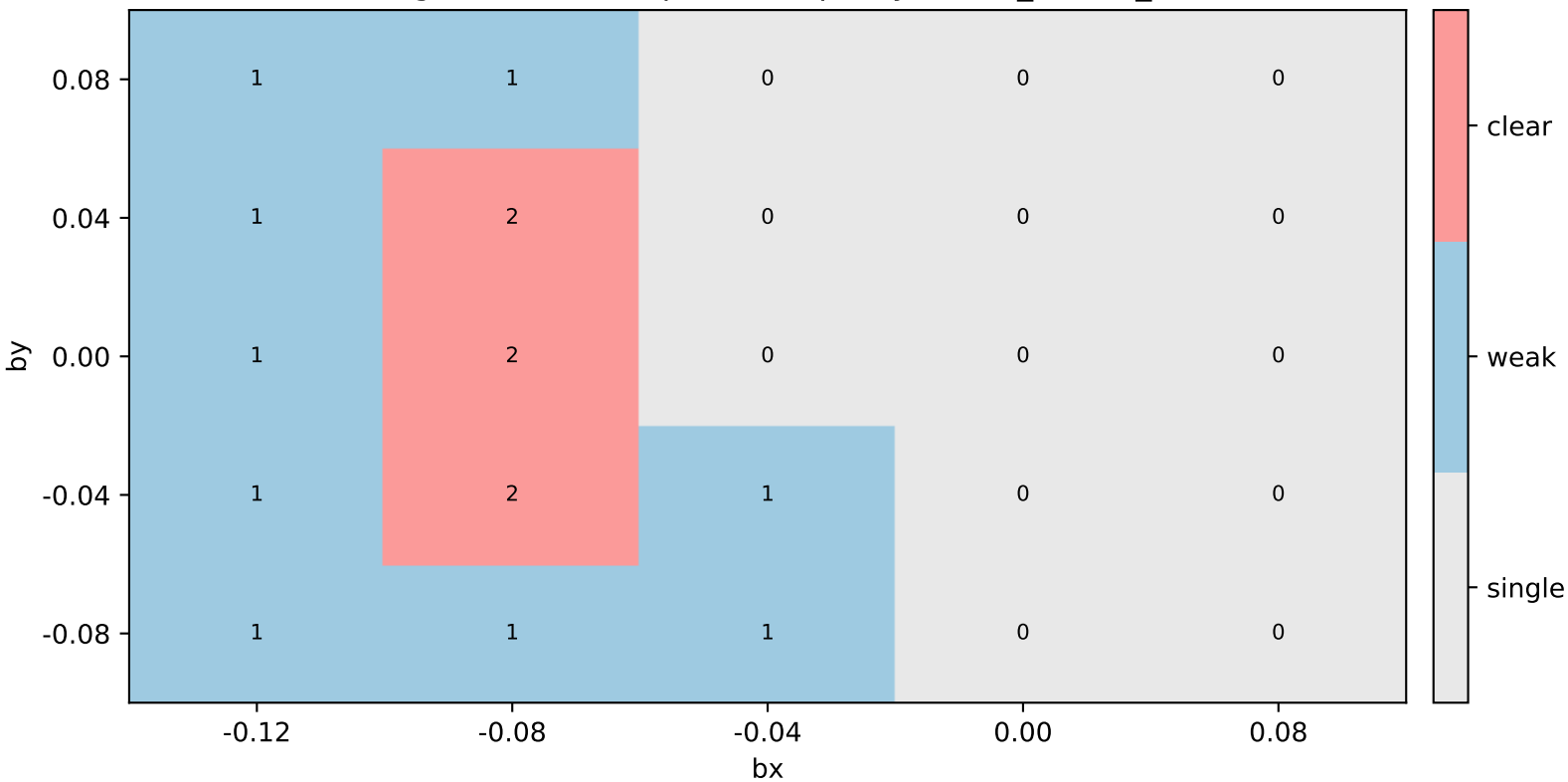
One-target bias-vector phase map (Wy=12, x_s=7, x_t=58)
