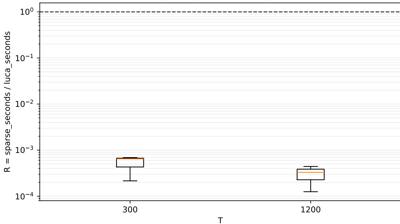
Speedup Distribution by T
